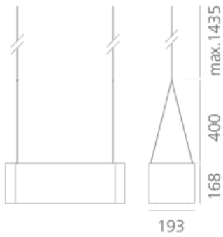
GREEN LIGHT_C
